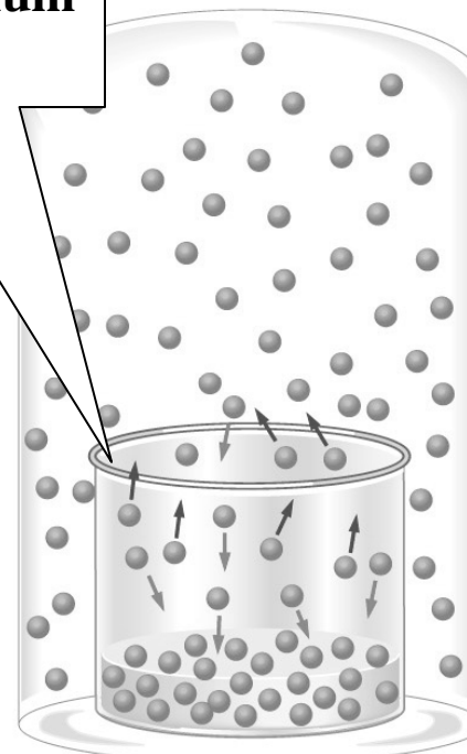
(c) Vaporization rate = condensation rate
